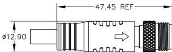
Male Plug
