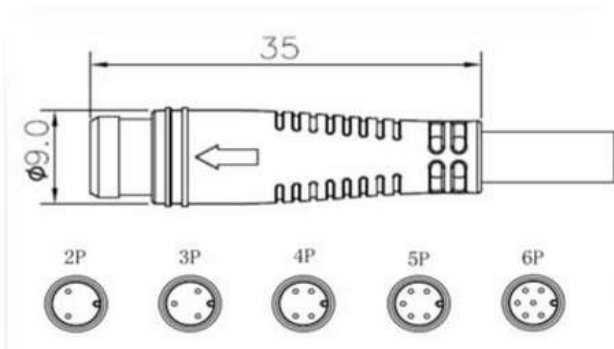
Male Plug
