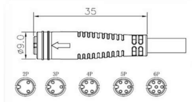
Female Plug
